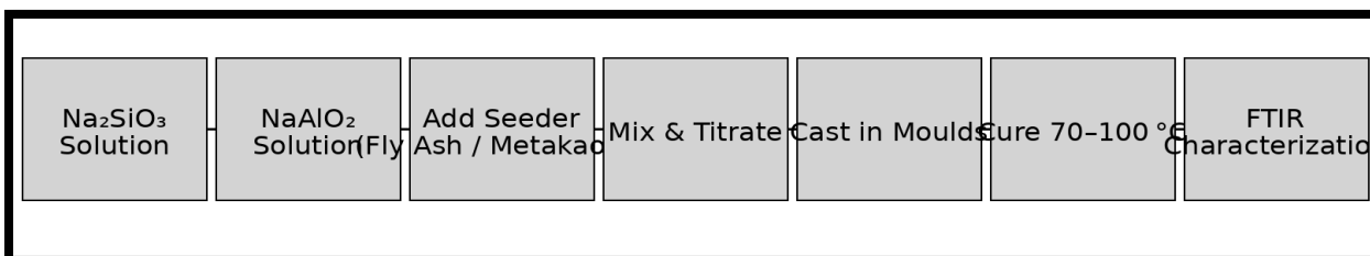
Figure 1. Schematic workflow of geopolymer resin synthesis from liquid precursors.
