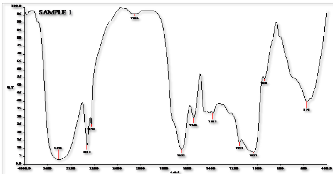
Fig 3: FTIR spectra of Anabaena sp.
