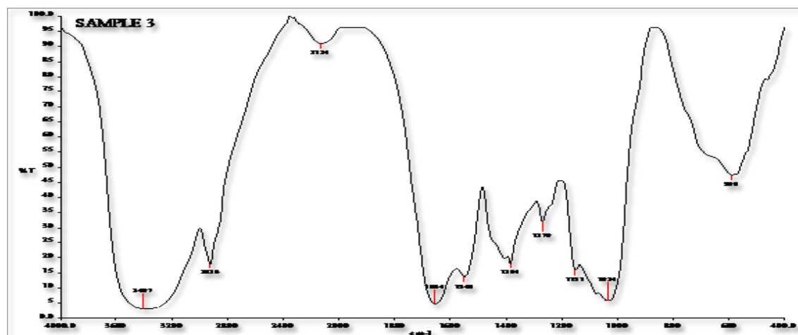
Fig 5 : FTIR spectra of phormidium sp.
