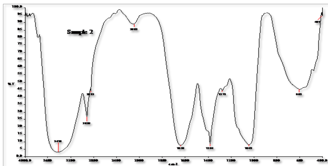
Fig. 4: FTIR spectra of Nostoc sp.
